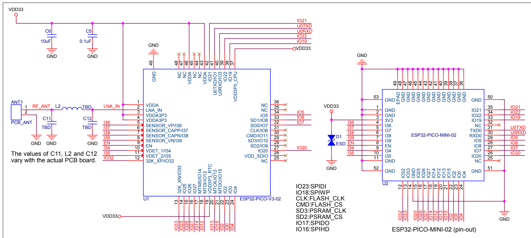
Figure 5: ESP32-PICO-MINI-02 Schematics
